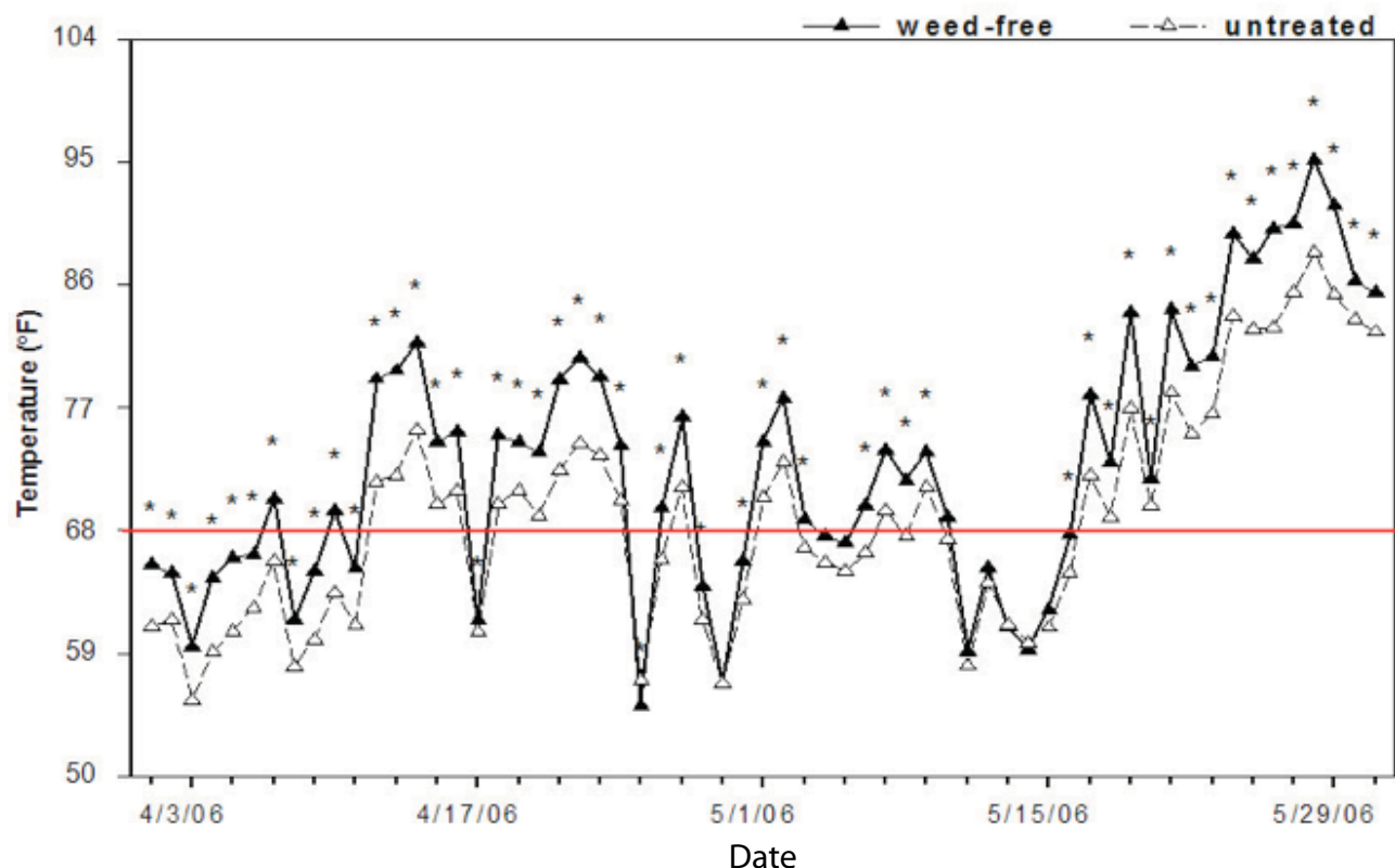
Figure 2. Influence of winter annual weed removal with fall herbicide applications on soil temperature prior to soybean planting as compared to untreated plots with a dense cover of winter annual weeds. Asterisks indicate significant differences in soil temperature within a day.
